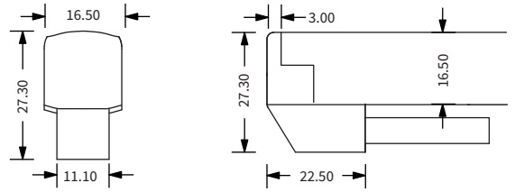
L Shape Entry Connector YYZ-MIC-LSEC-01 (Single Feed-Right Side) YYZ-MIC-LSEC-02 (Single Feed-Left Side) YYZ-MIC-LSEC-03 (Double Feed-Both Side)
