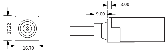
Direct Entry Connector YYZ-MIC-DEC-01 (Single Feed-Right Side) YYZ-MIC-DEC-02 (Single Feed-Left Side) YYZ-MIC-DEC-03 (Double Feed-Both Side)
