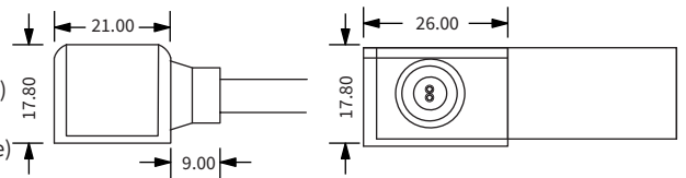
Side Entry Connector YYZ-MIC-SEC-01 (Single Feed-Right Side) YYZ-MIC-SEC-02 (Single Feed-Left Side) YYZ-MIC-SEC-03 (Double Feed-Both Side)
