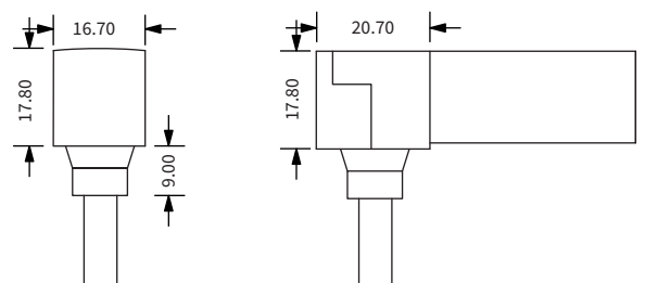
Bottom Entry Connector YYZ-MIC-BEC-01 (Single Feed-Right Side) YYZ-MIC-BEC-02 (Single Feed-Left Side) YYZ-MIC-BEC-03 (Double Feed-Both Side)
