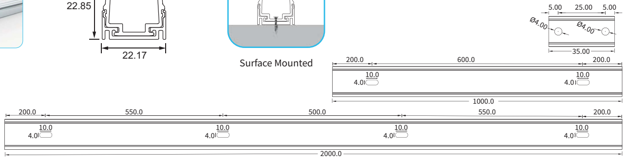
Installation Way
