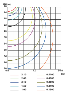
C0 PLANE ISOLUX DIAGRAM (UNIT:lx)
