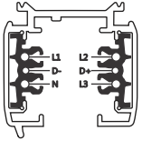
Surface mounted track
